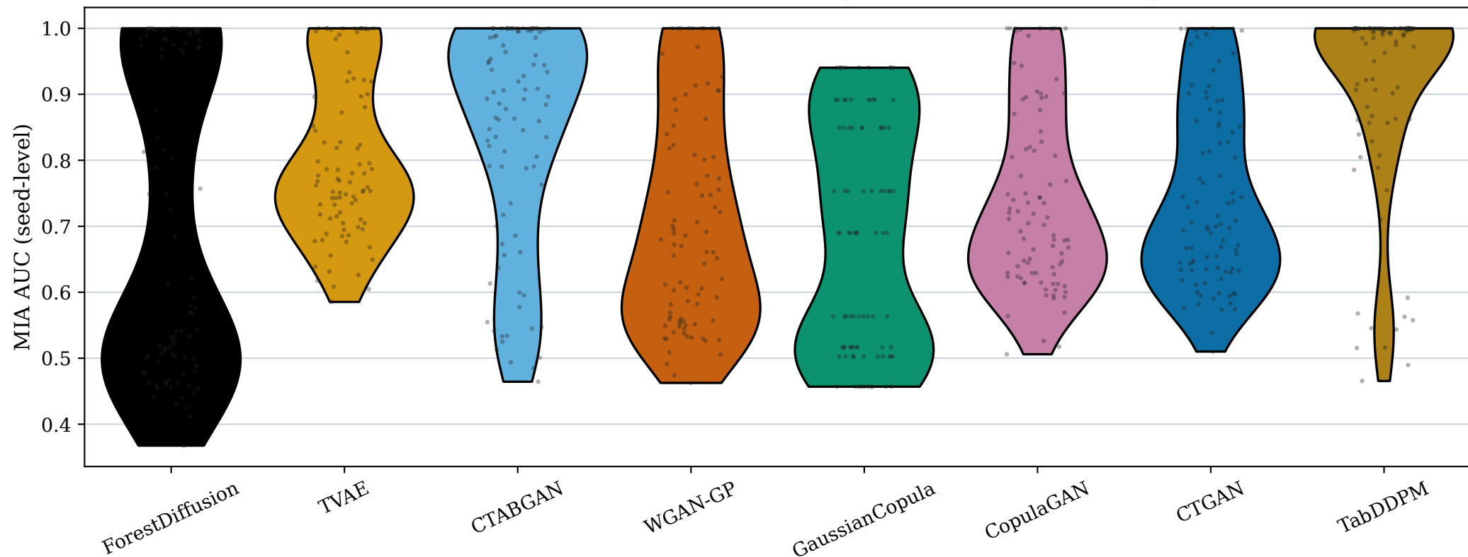
MIA AUC — seed-level distribution (n = 10 seeds × datasets)
